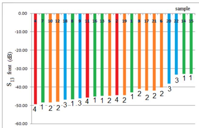
Figure 10. Scatter coefficient in descending order with noted sample categories
