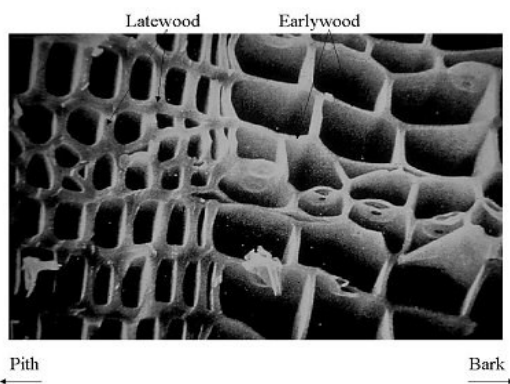
Figure 1. Microscopic image of Earlywood Latewood Structure
