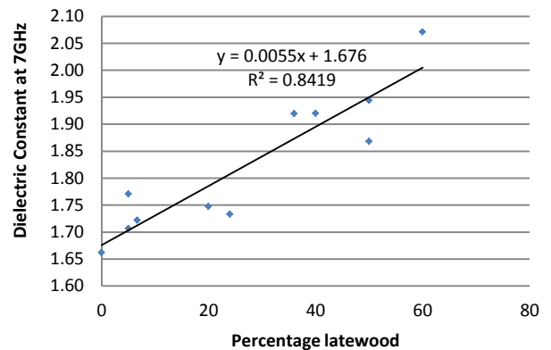
Figure 4. Measured Dielectric constant at 7GHz versus percentage late wood in the sample
