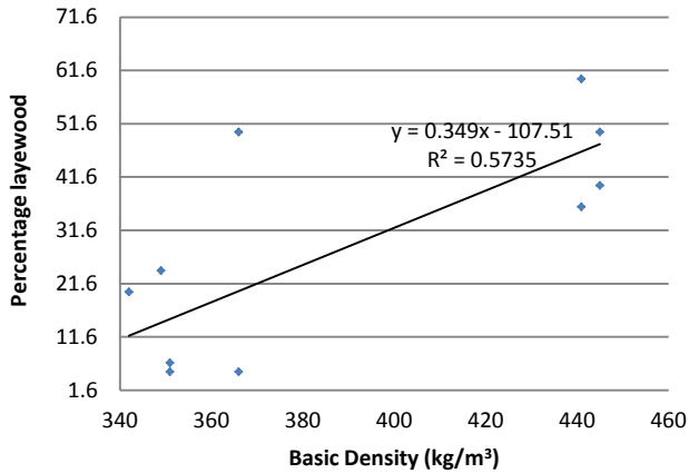
Figure 6. Percentage Latewood versus Basic Density
