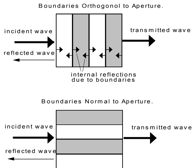
Figure 2. EW/LW layering
