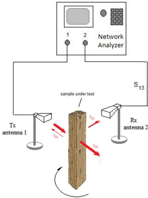
Figure 8. Measurement setup
