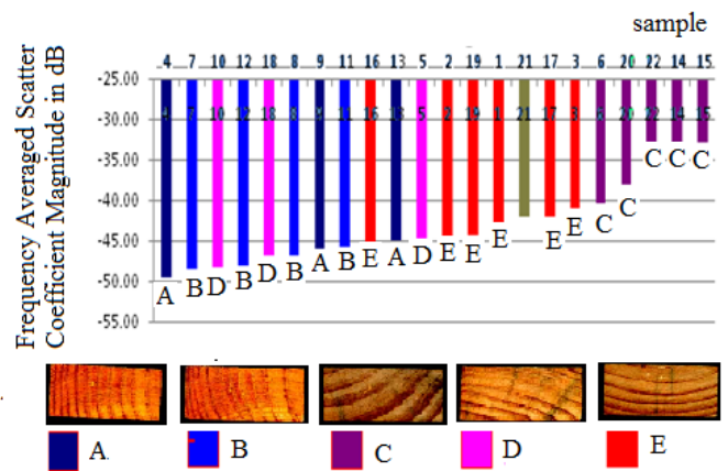
Figure 11. Frequency Averaged Scatter Coefficient Magnitudes and samples grouped by the annual ring pattern
