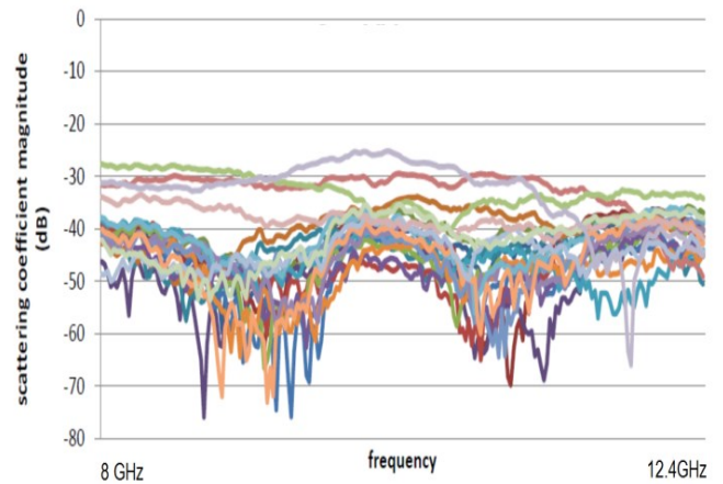
Figure 9. Scatter coefficient S_{13} magnitudes vs. frequency (8 to 12.4 GHz range) for twenty two samples, measured in nominal vertical polarization
