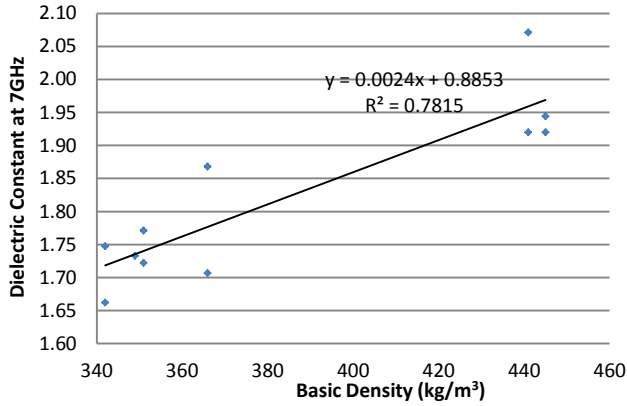
Figure 5. Measured Dielectric constant at 7GHz versus Basic Density
