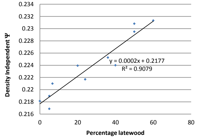
Figure 7. Density Independent Factor at 7GHz versus Percentage Late wood
